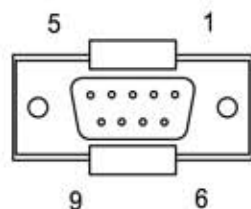
ATD9FCK FEMALE
